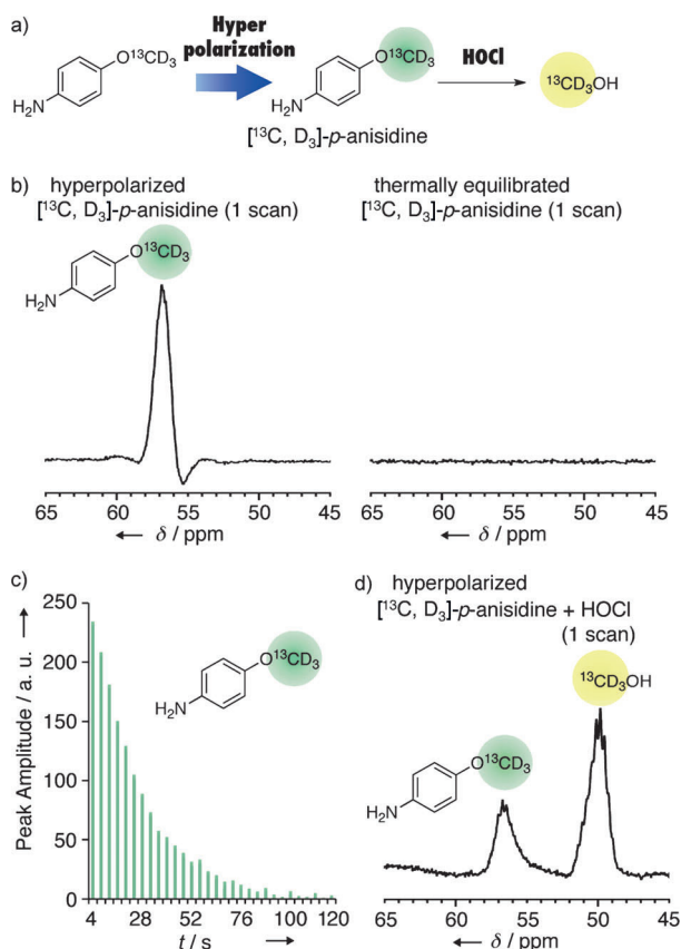
Figure 3. a) Illustration of experimental procedures. b) ^{13}\text{C} NMR spectra of hyperpolarized (4 s after rapid dissolution, left) and thermally equilibrated (right) [^{13}\text{C},\text{D}_3]\text{-}p\text{-anisidine} (10 mM). c) Time-resolved ^{13}\text{C} NMR data of hyperpolarized [^{13}\text{C},\text{D}_3]\text{-}p\text{-anisidine} (1.7 mM). The peak amplitude of [^{13}\text{C},\text{D}_3]\text{-}p\text{-anisidine} was plotted from 4 to 120 s after initiation of the NMR acquisition. d) ^{13}\text{C} NMR spectrum of hyperpolarized [^{13}\text{C},\text{D}_3]\text{-}p\text{-anisidine} (10 mM) observed 4 s after addition of \text{HOCl} (20 mM). NMR spectra were measured with a 7.05 T NMR instrument with 90^\circ (b,d) and 18^\circ pulse angles (c).
